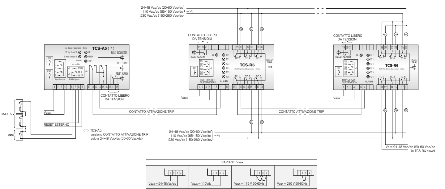
Example of circuit breaker opening system with TCS-A5 and TCS-R6 modules
