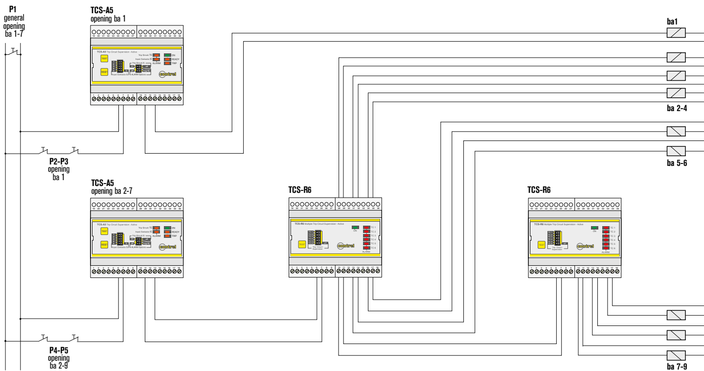
Example of circuit breaker opening system with TCS-A5 and TCS-R6 modules
