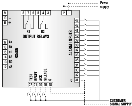
COMPALARM C2C Higher Voltage Powered Inputs
